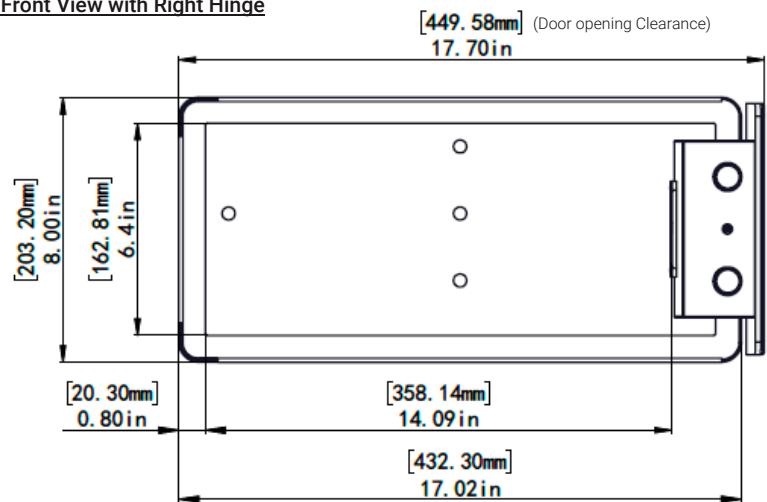
Front View with Right Hinge
